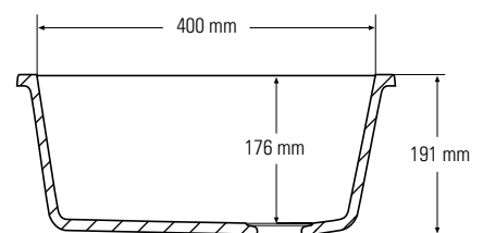
Side cross-section
