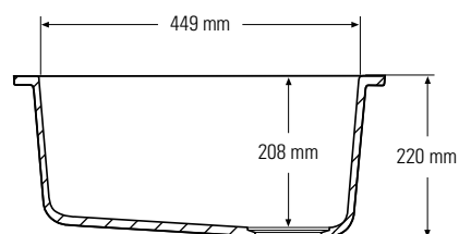
Side cross-section
