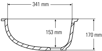
Side cross-section
