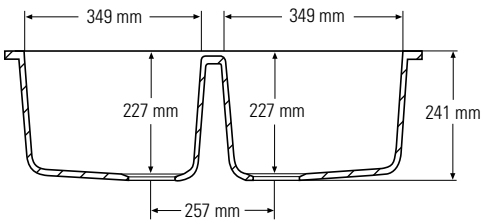
Front cross-section
