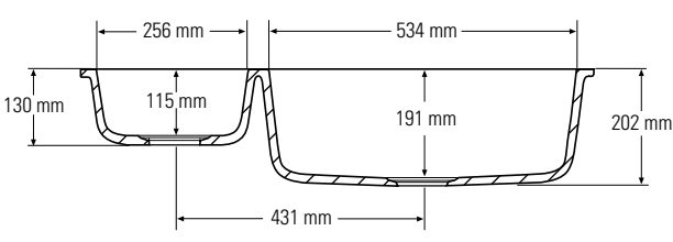
Front cross-section
