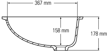
Side cross-section
