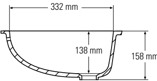
Side cross-section
