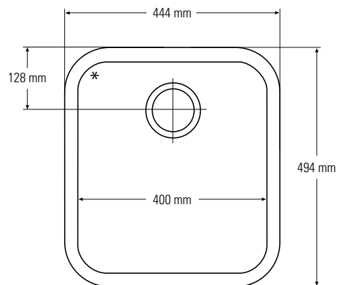
Top view * overflow
